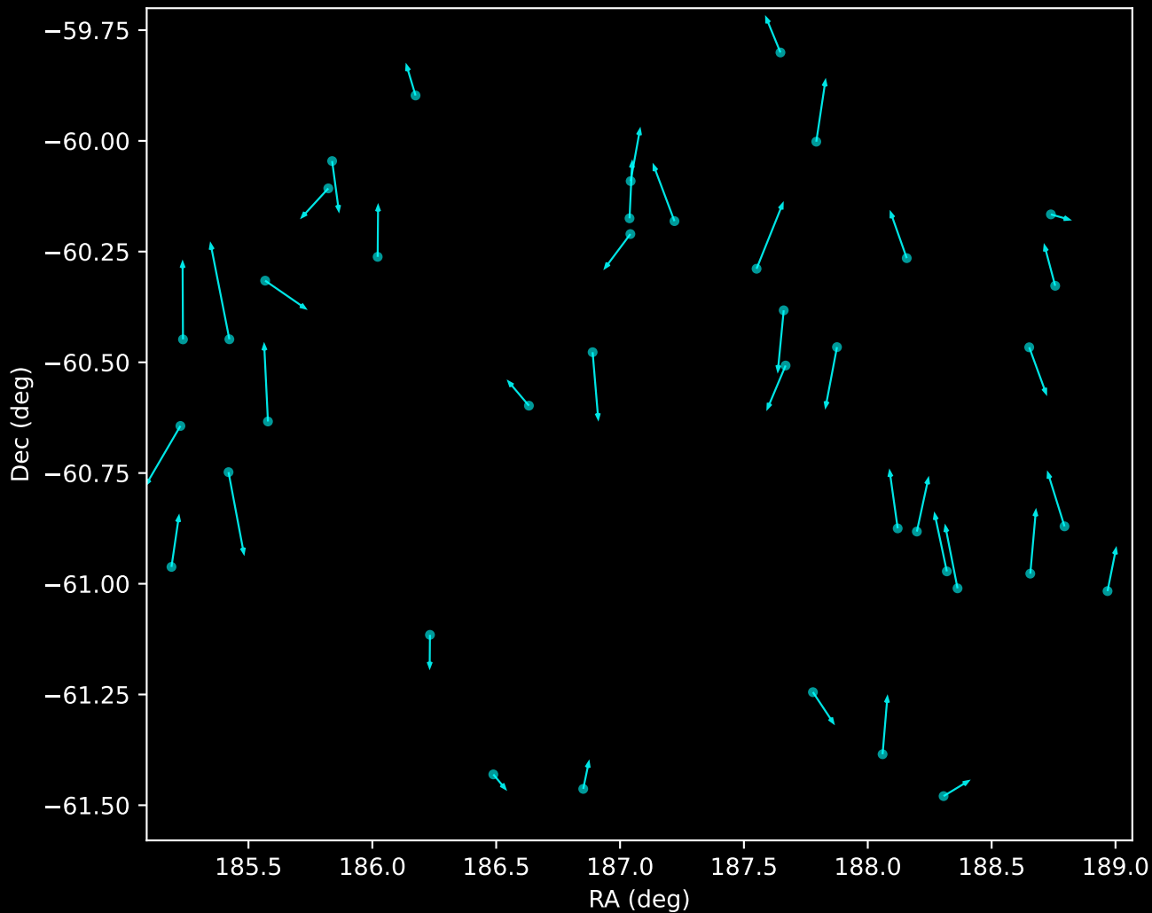
GALAH DR4 Noise Stream Proper Motion Vectors (n=40)
