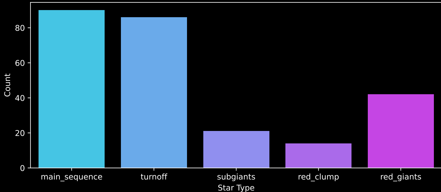
GALAH DR4 Field: [7140] Count plot of Star Type
