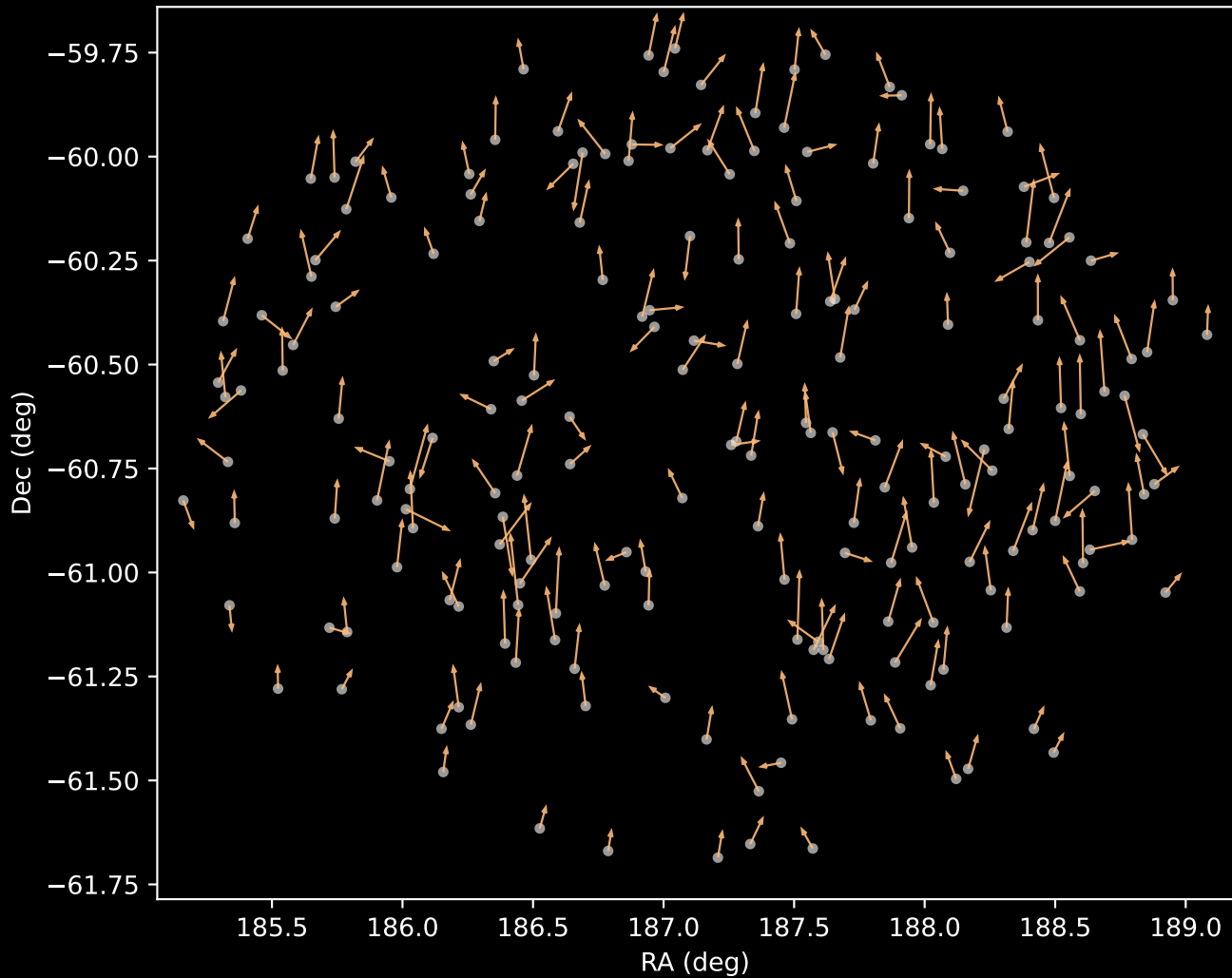
GALAH DR4 Cluster 3 Proper Motion Vectors (n=195)
