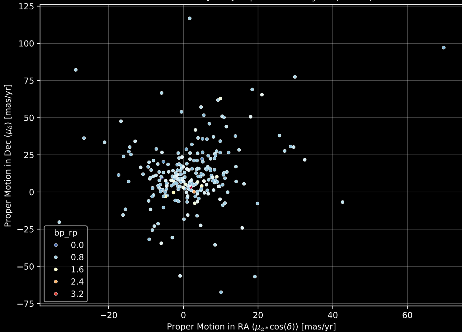
GALAH DR4 Field: [7140] Proper Motion Diagram (n= 253)
