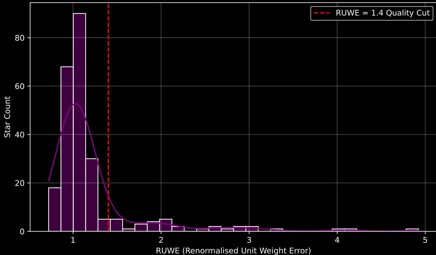
GALAH DR4 Field [7140] RUWE Distribution (n= 243)
