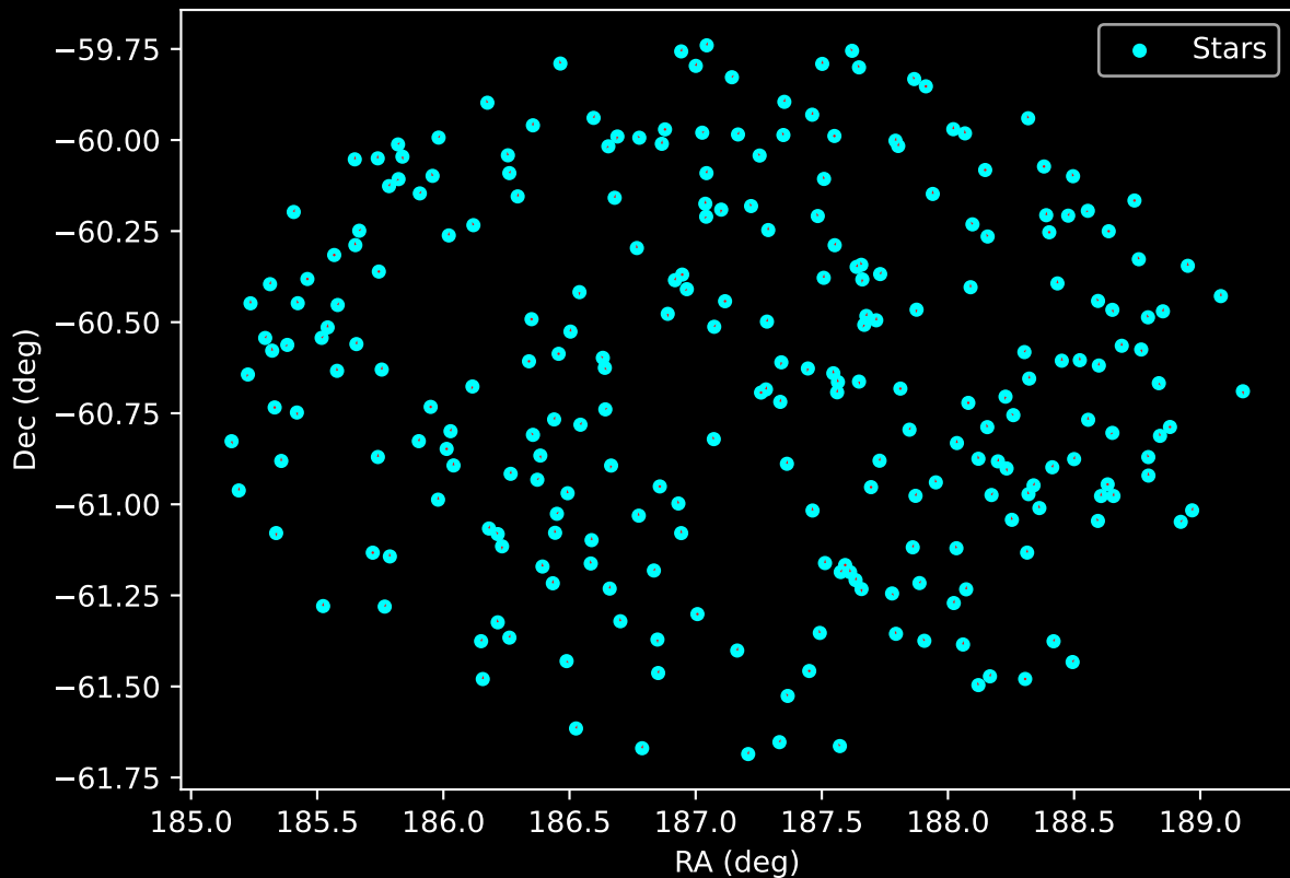
GALAH DR4 Field: [7140] Proper Motion Vectors for Gaia Star Field (n= 253)
